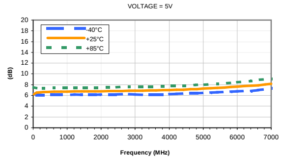
NOISE FIGURE vs. FREQUENCY & TEMPERATURE
