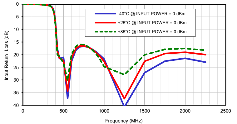
Input Return Loss vs. Temperature
