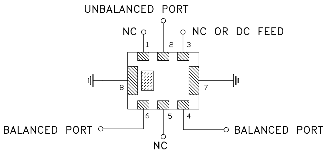
Schematic Diagram
