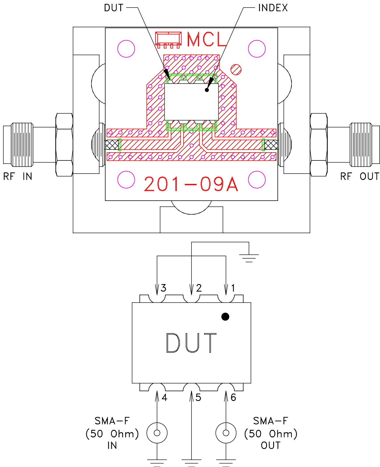
Schematic diagram
