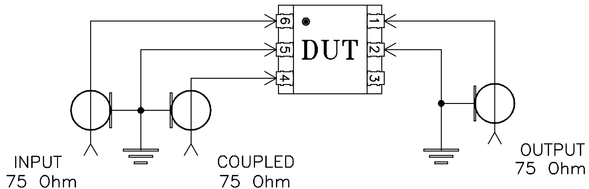
Schematic Diagram
