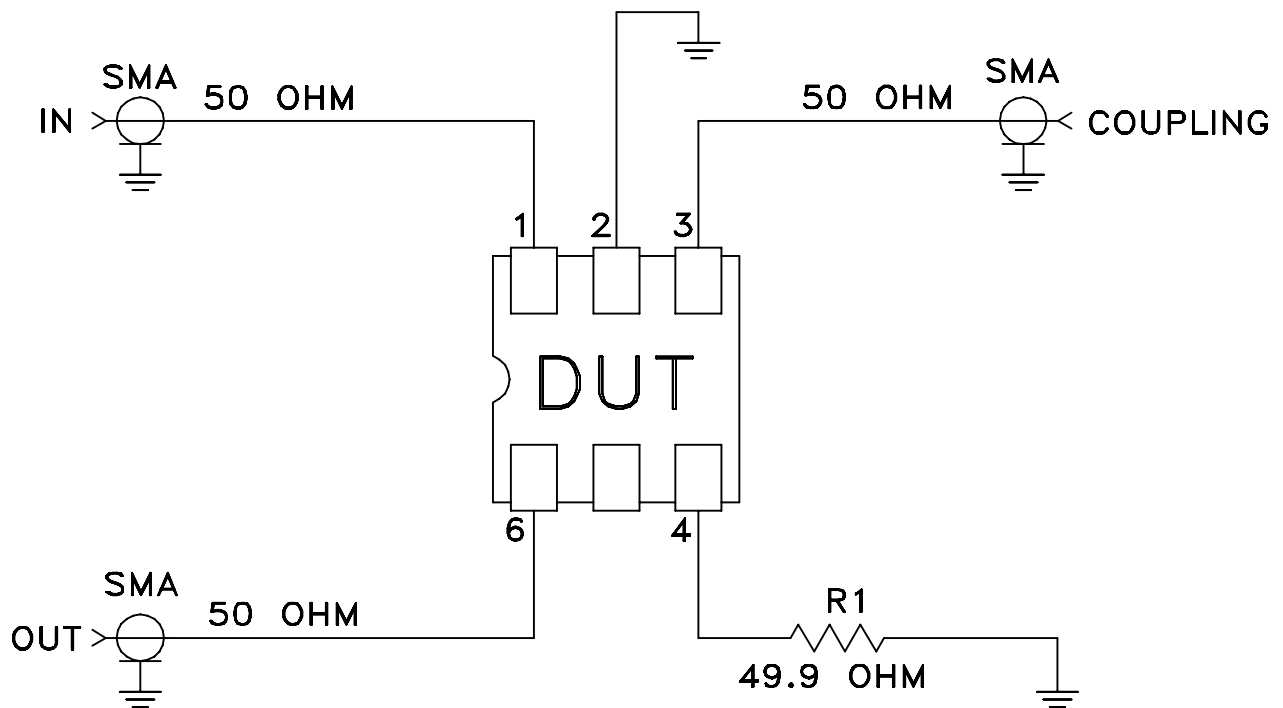
Schematic Diagram
