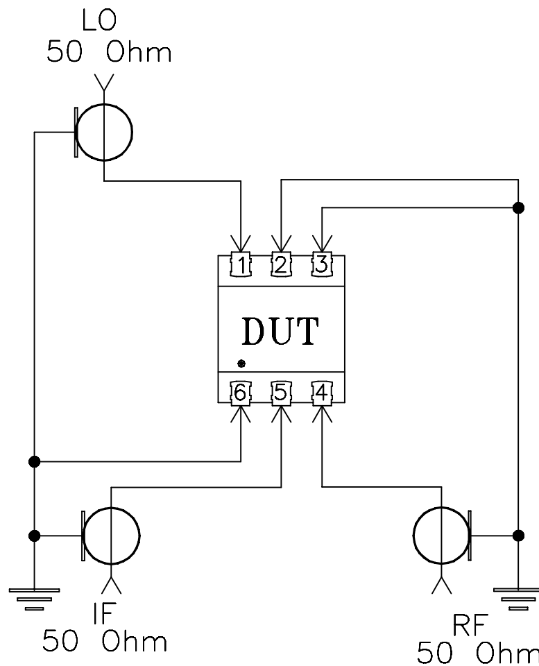
Schematic Diagram
