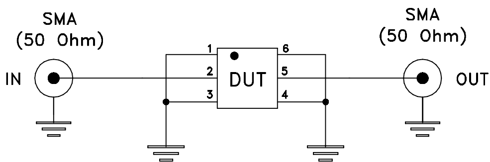
Schematic Diagram
