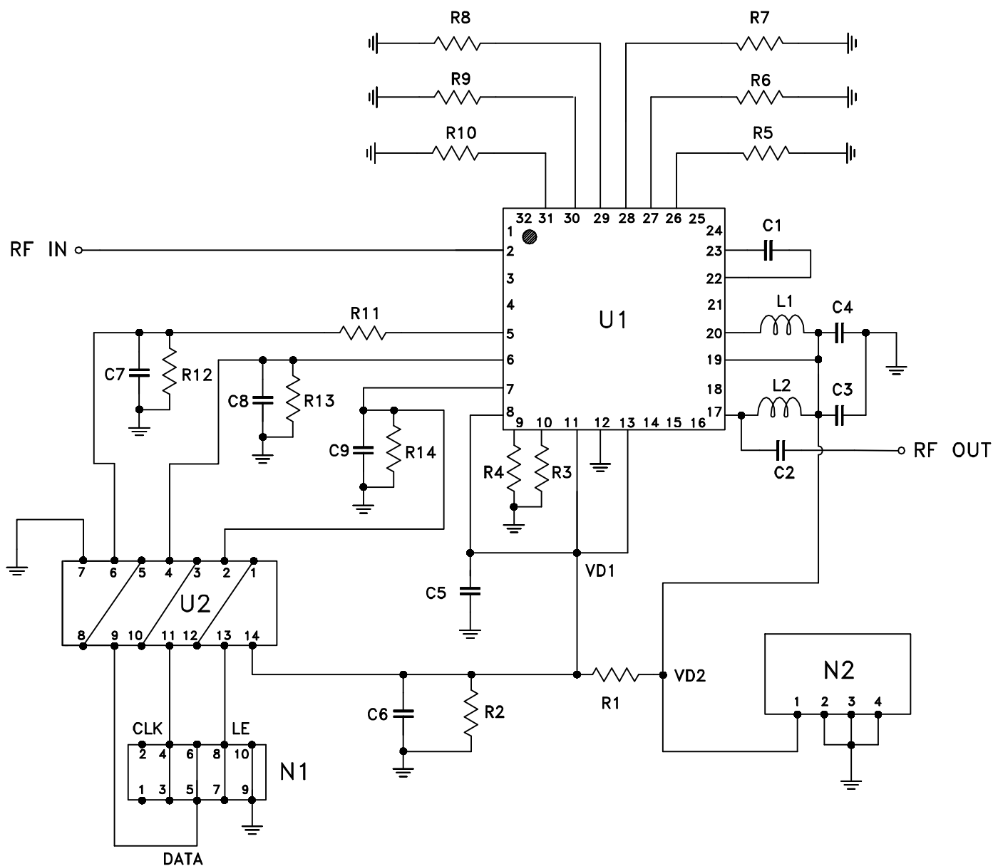
Schematic Diagram
