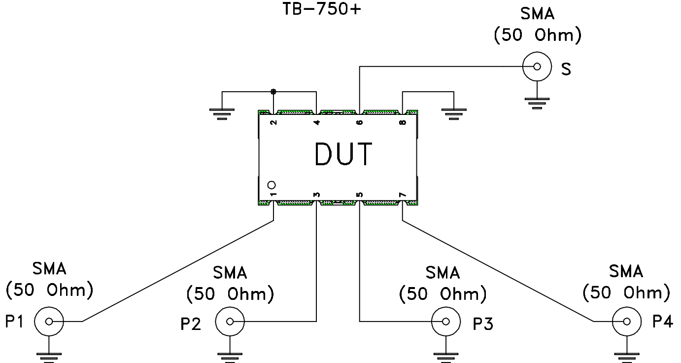
Schematic Diagram
