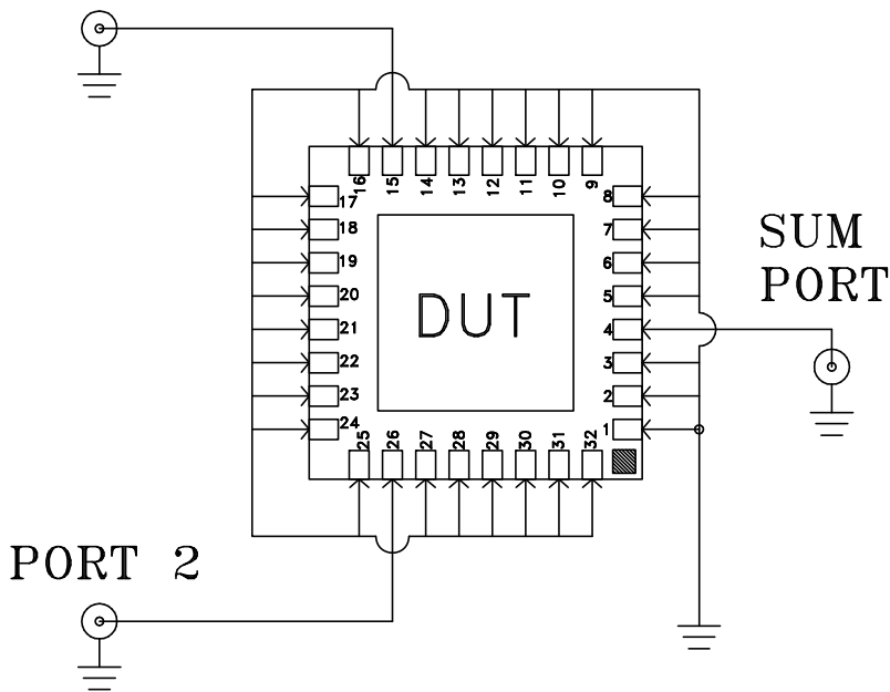
SCHEMATIC DIAGRAM
