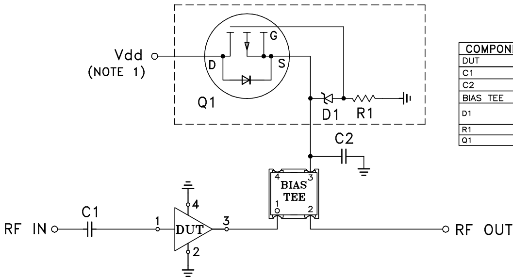
Schematic Diagram
