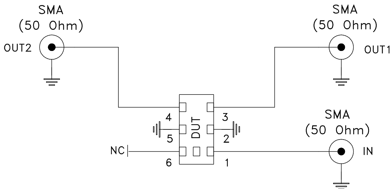
Schematic Diagram
