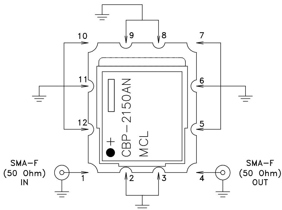
Schematic diagram
