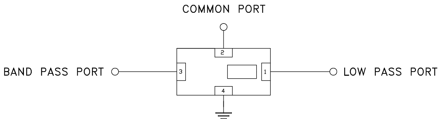
Schematic Diagram
