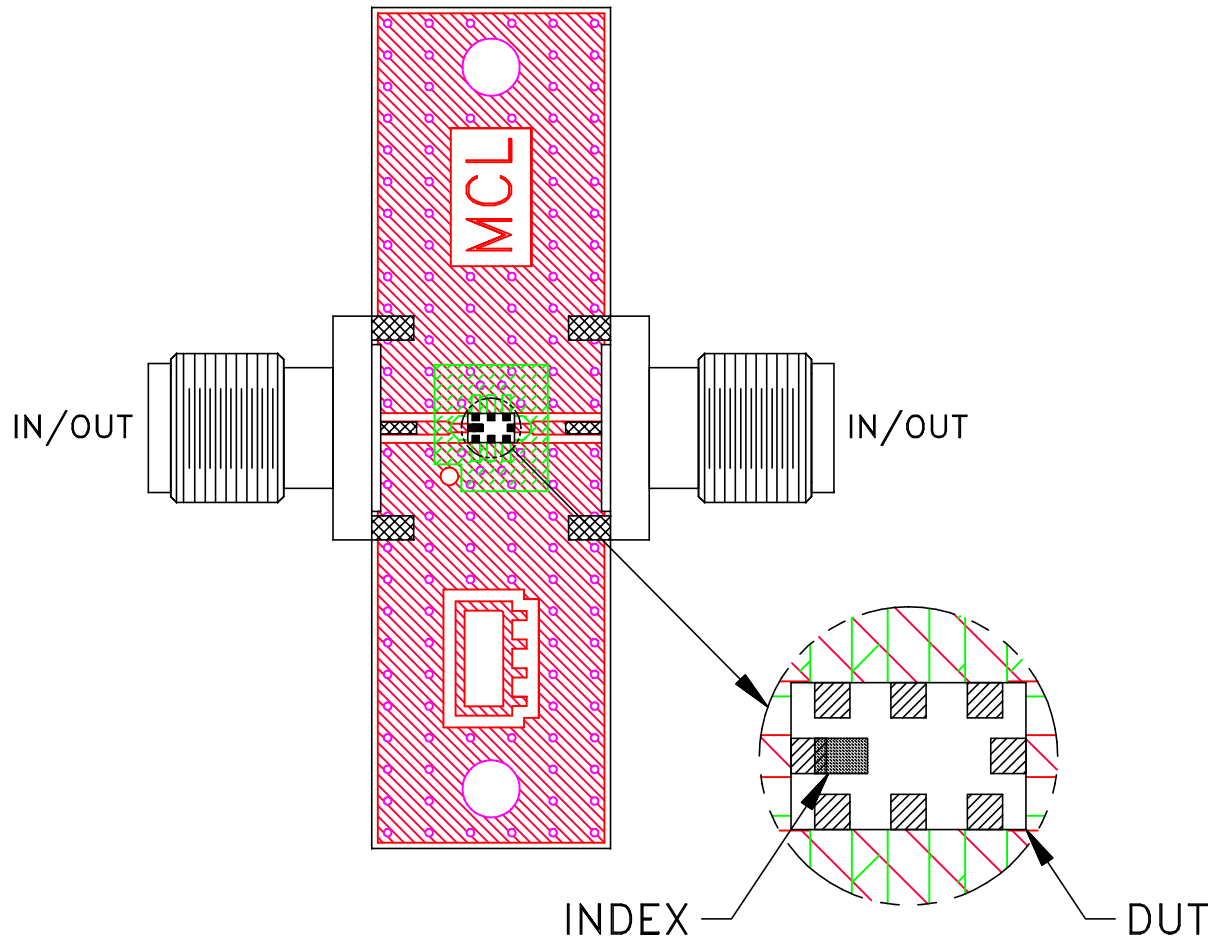
Schematic diagram
