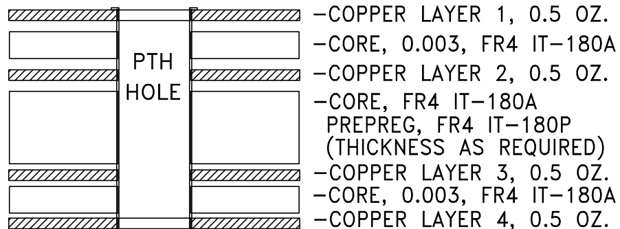
Stack-up Diagram
