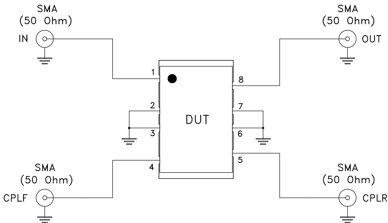
Schematic Diagram
