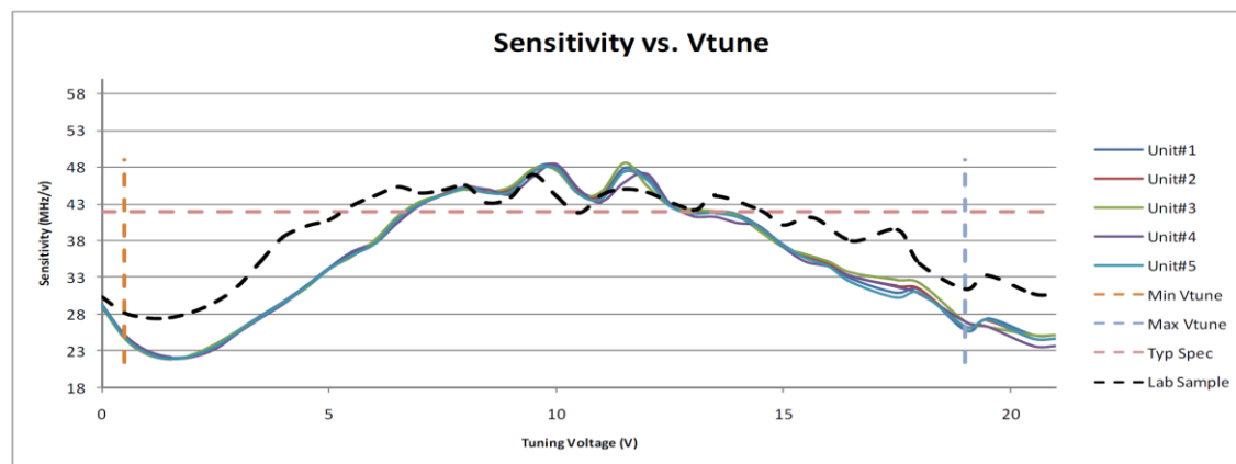
Figure 3: Sens. @ Nom Vcc [MHz/V] vs. Vtune [V] at +25°C
