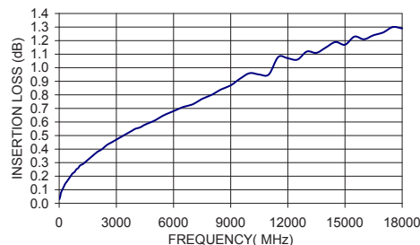
086-14SM+ INSERTION LOSS
