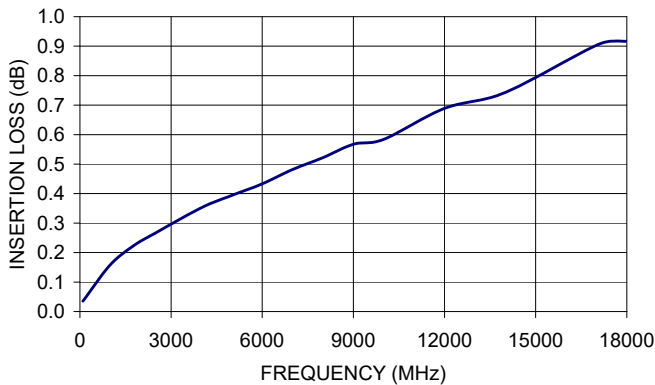
141-15SMRSM+ INSERTION LOSS
