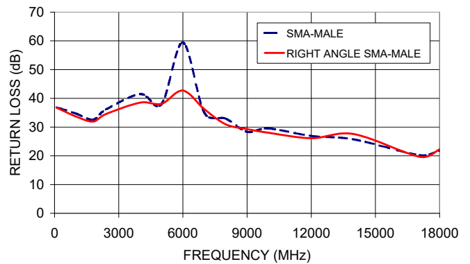
141-15SMRSM+ RETURN LOSS
