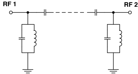
Figure 1. ABF-16G+ Functional Diagram
