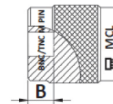
Fig 3. Gaging a Male BNC/TNC Connector
