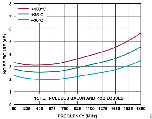
Figure 21. Noise Figure vs. Frequency over Temperature
