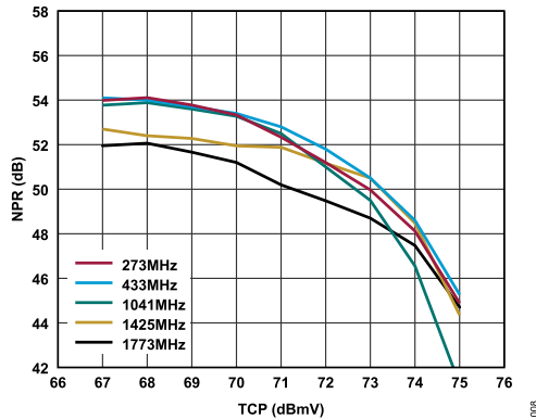
Figure 7. NPR vs. TCP over Frequency, 20 dB Tilt
