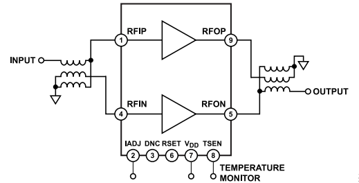
Figure 1. Functional Block Diagram
