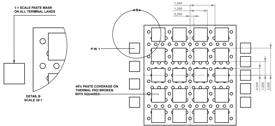
Figure 23. Recommended Solder Pattern (Dimensions Shown in Millimeters)
