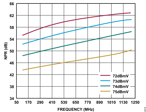
Figure 13. NPR vs. Frequency over TCP, 13 dB Tilt
