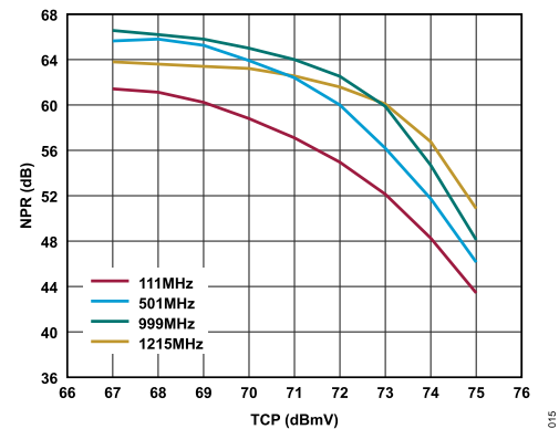
Figure 14. NPR vs. TCP over Frequency, 13 dB Tilt
