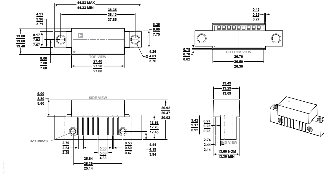
Figure 12. 8-Pin SOT115J Module Package [MODULE] (ML-8-1)
