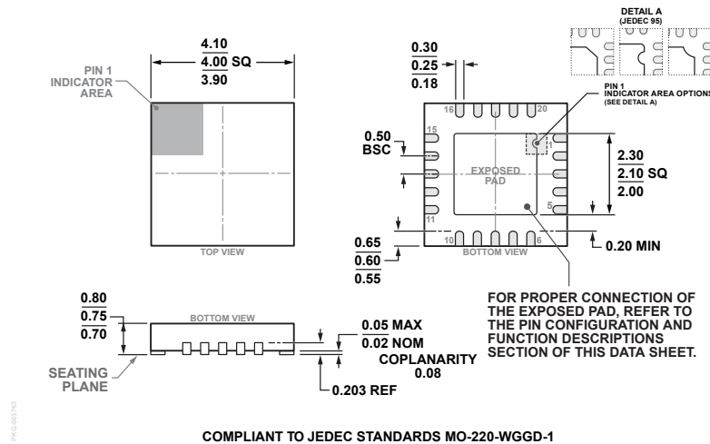
Figure 40. 20-Lead Lead Frame Chip Scale Package [LFCSP] 4 mm × 4 mm Body and 0.75 mm Package Height (CP-20-6)
