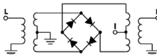
Electrical Schematic
