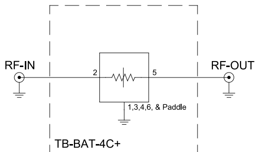
Figure 2. BAT-4+ Characterization and Application Circuit.
