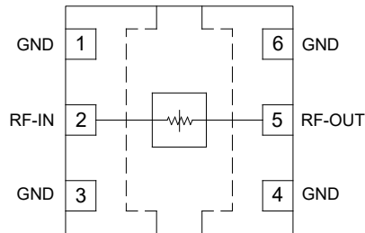
Figure 1. BAT-8+ Functional Diagram
