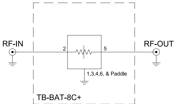
Figure 2. BAT-8+ Characterization and Application Circuit.
