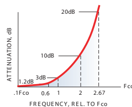
TYPICAL FREQUENCY RESPONSE INSERTION LOSS
