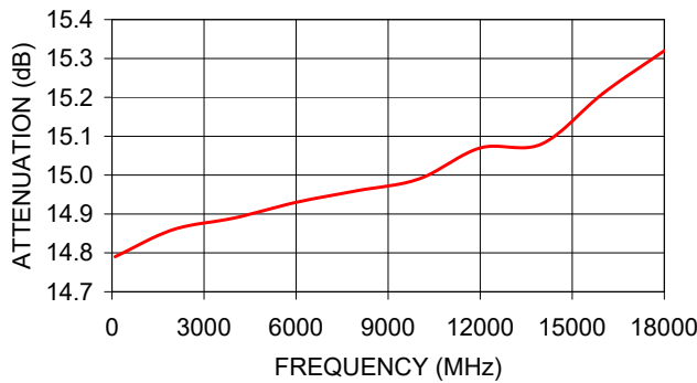
BW-S15W5+ ATTENUATION
