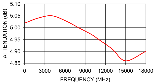
BW-S5W5+ ATTENUATION
