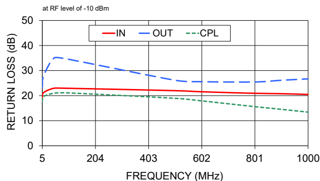
RETURN LOSS
