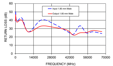
E67-1M-EMEM+ RETURN LOSS
