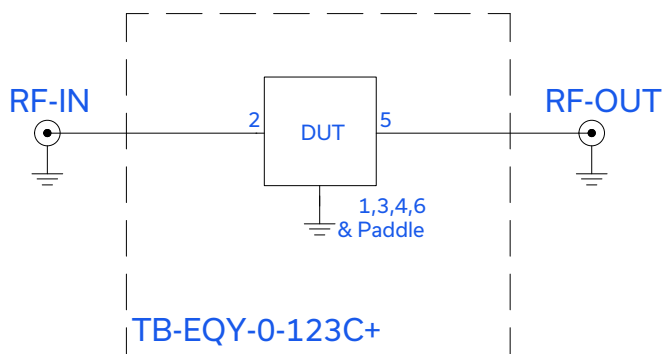
Figure 2. EQY-0-123C+ Evaluation and Application Circuit
