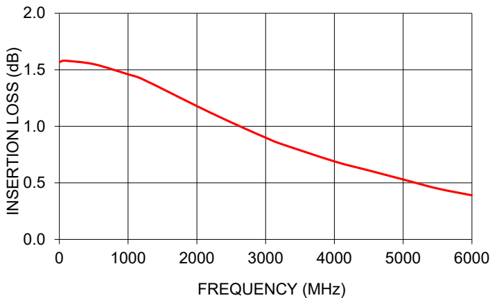
EQY-1-63+ INSERTION LOSS
