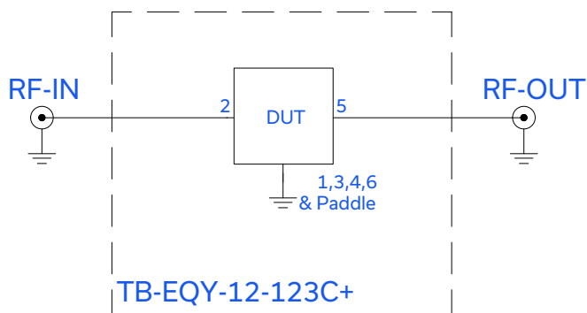
Figure 2. EQY-12-123C+ Evaluation and Application Circuit
