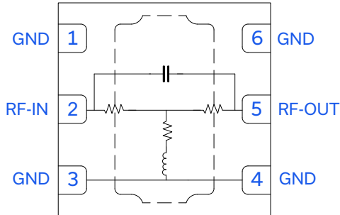
Figure 1. EQY-5-123+ Functional Diagram
