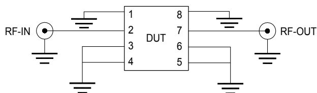
Fig 1. Block Diagram of Test Circuit used for characterization. Test Board TB-EQY-8-24+
