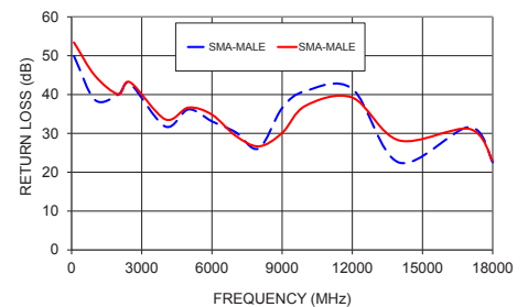
FL086-6SM+ RETURN LOSS
