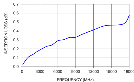
FL086-6SM+ INSERTION LOSS
