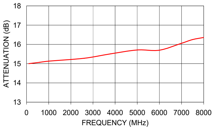
GAT-15+ ATTENUATION
