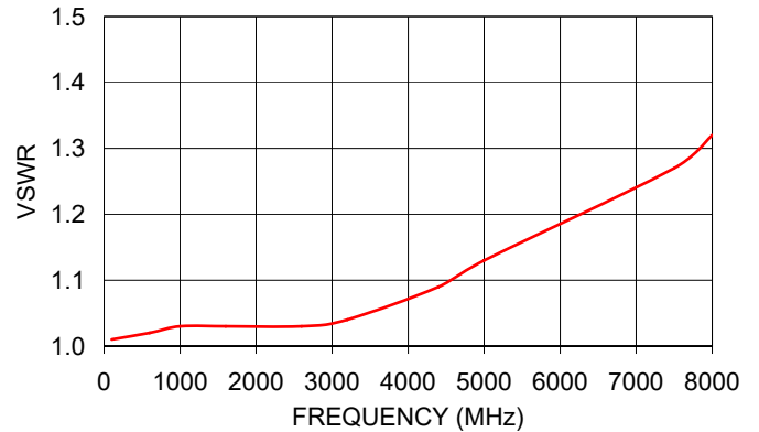
GAT-20+ VSWR
