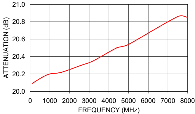
GAT-20+ ATTENUATION
