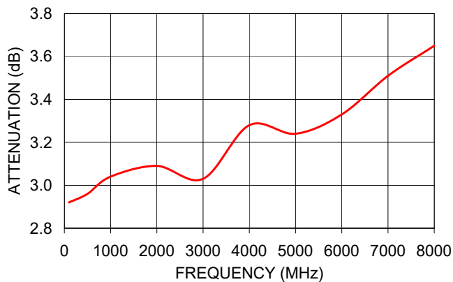
GAT-3+ ATTENUATION
