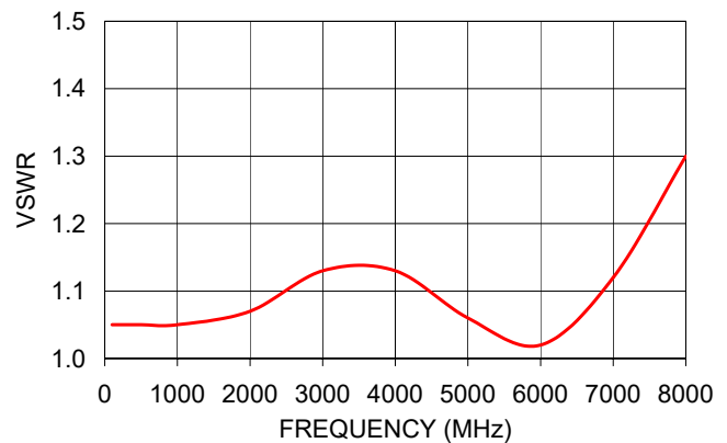
GAT-3+ VSWR
