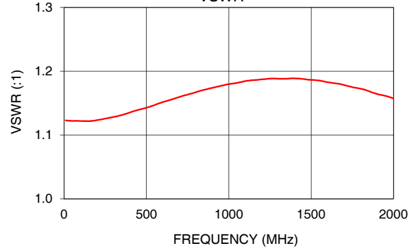
HAT-15A+ VSWR
