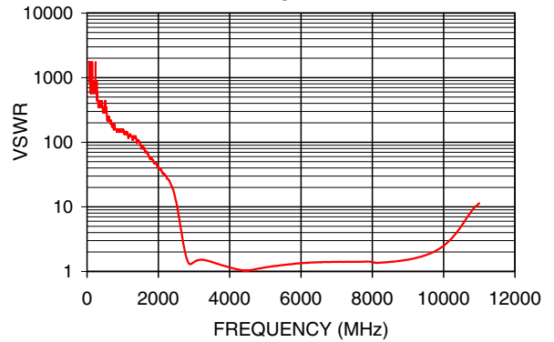
HFCN-2700AD+ VSWR
