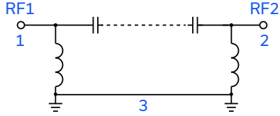
Figure 1. HFHKI-2000+ Functional Diagram
