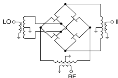
Electrical Schematic
