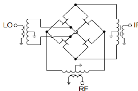
Electrical Schematic
