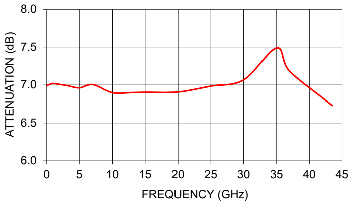
KAT-7+ ATTENUATION
