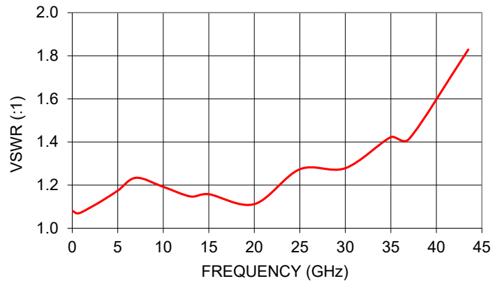
KAT-7+ VSWR
