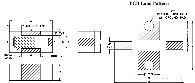
Suggested Layout, Tolerance to be within ±.002
